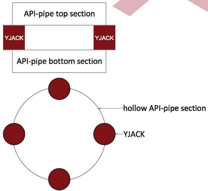
YJACK Type M for Cast In-Situ API-Micro Piles (mini or micro piles with API-pipe as reinforcement)
